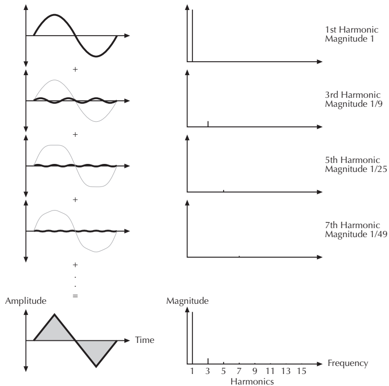
Additive components of the Triangle wave
