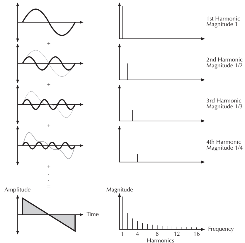
Additive components of the Sawtooth wave
