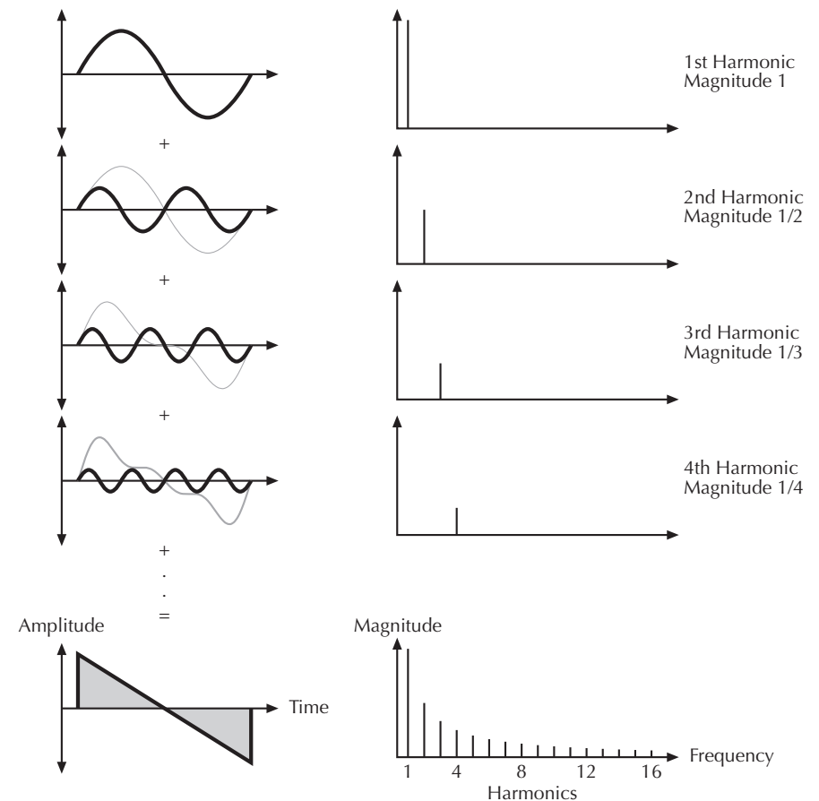
Additive components of the Sawtooth wave
